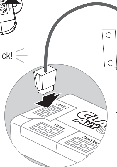
From your controls connect Green Harness into Control Port on ECU
